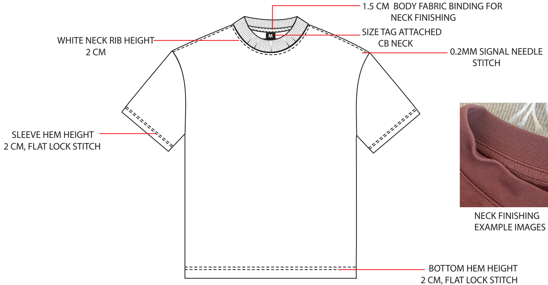
FRONT VIEW
